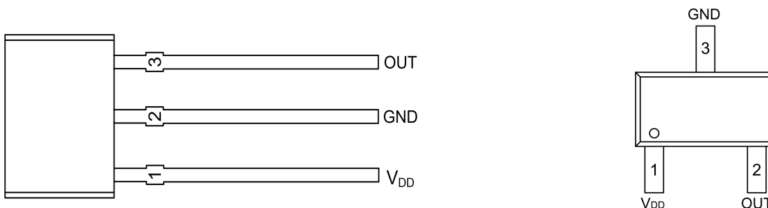
Figure 1, Pin Assignments of OCH1902
