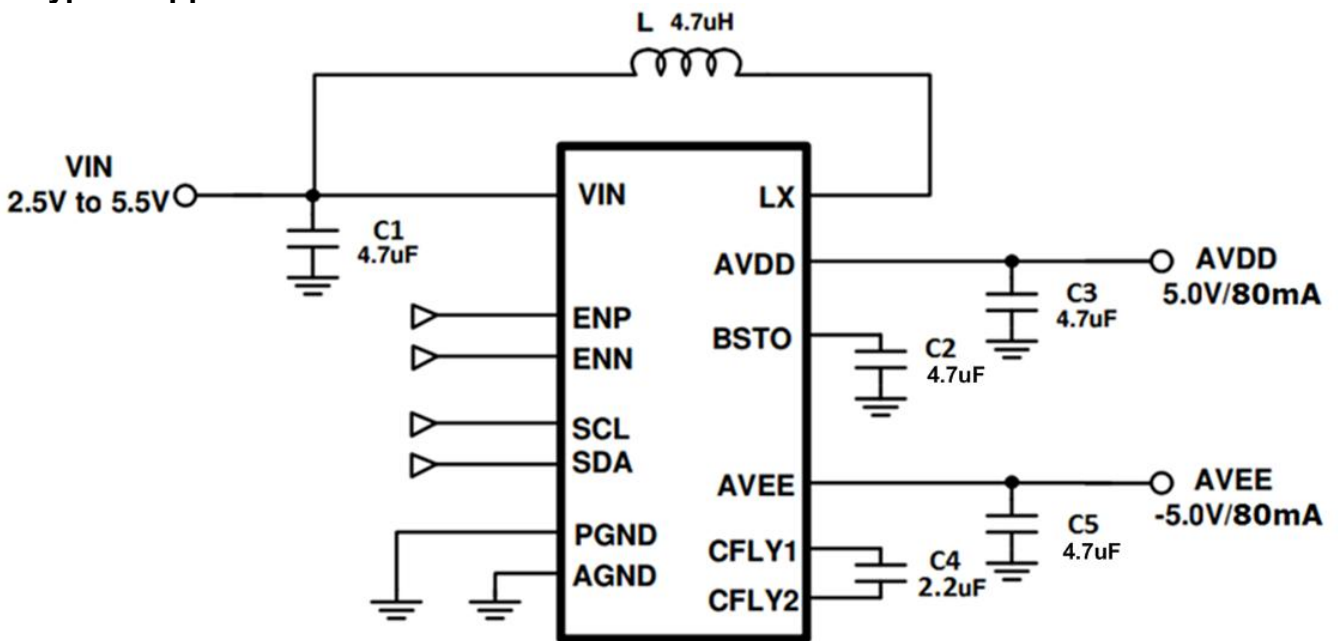
Figure 2, Typical Application Circuit of OCP2130
