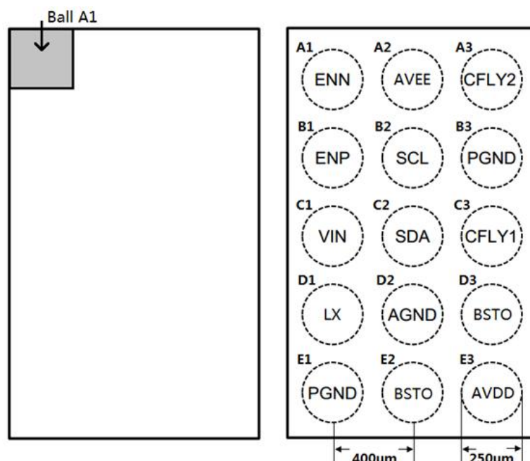
Figure 1, Pin Assignments of OCP2130
