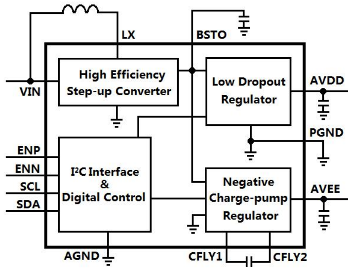
Figure 3, Block Diagram of OCP2130
