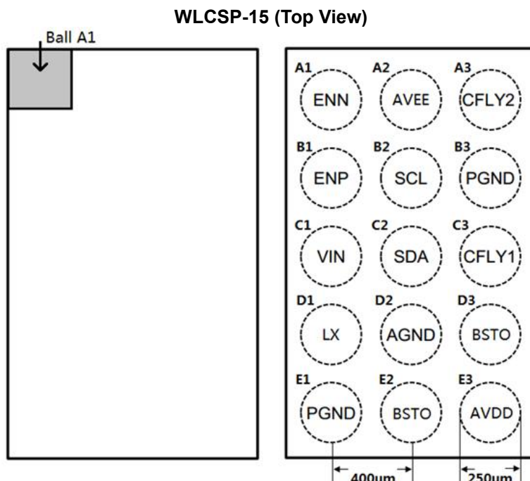
Figure 1, Pin Assignments of OCP2131
