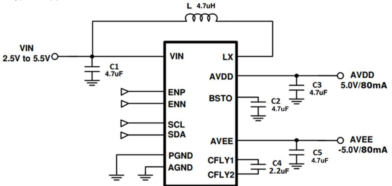
Figure 2, Typical Application Circuit of OCP2131
