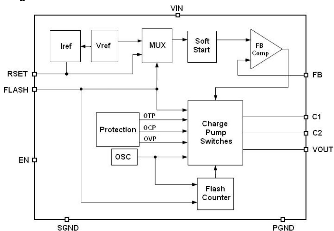
Figure 3, Block Diagram of OCP8111A
