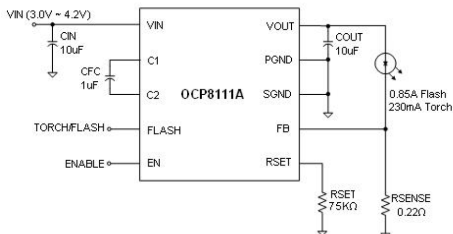
Figure 2A, Typical Application Circuit of OCP8111A
