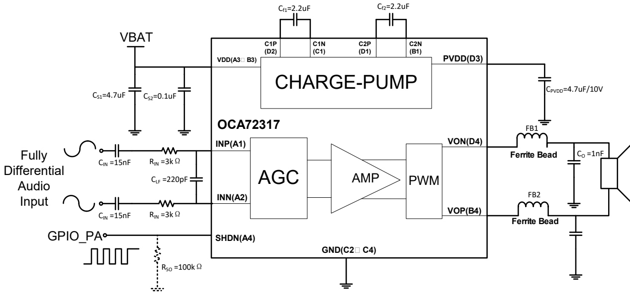
Figure 5. Fully-differential application
