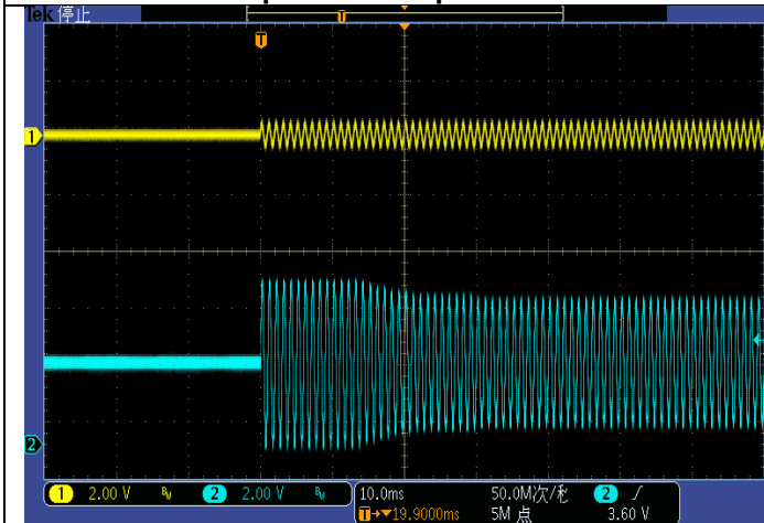
AGC Start-up Waveform CH1:Input CH2:Output
