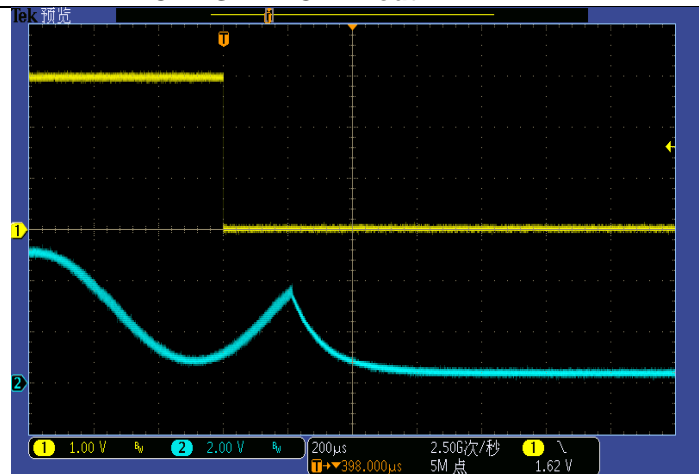
AGC Shut-down Waveform CH1:Input CH2:Output
