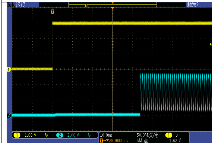
AGC Start-up Waveform CH1:Input CH2:Output
