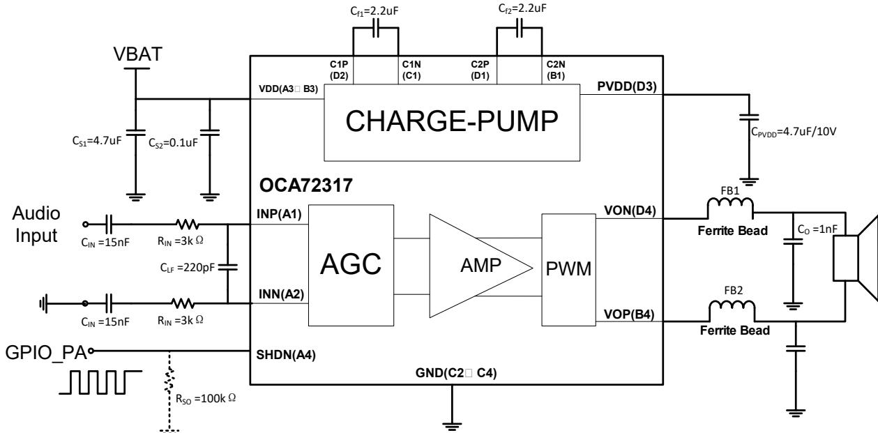
Figure 4. Single-ended application
