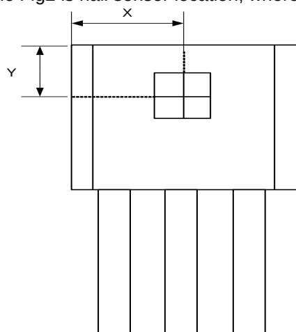
Fig2 OCH145 Hall Sensor Location
