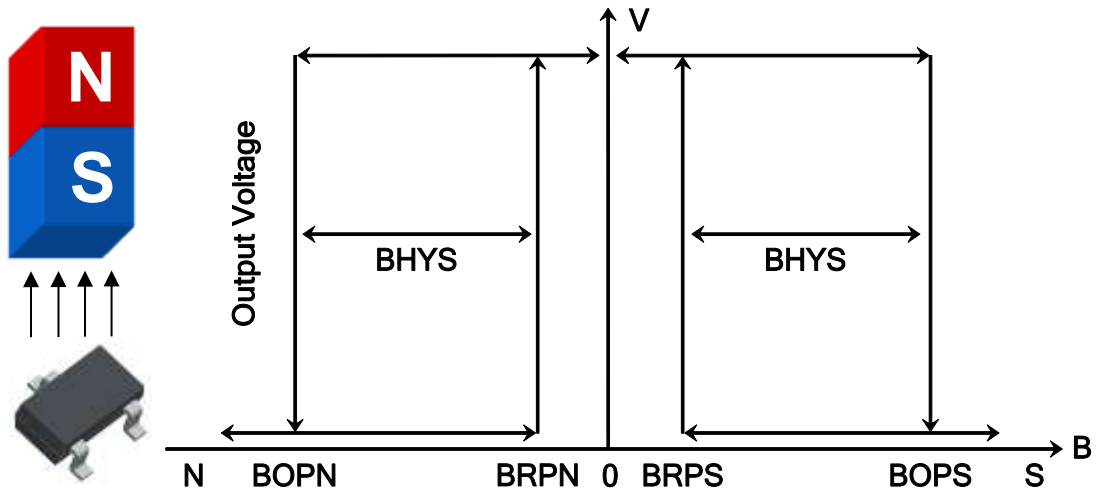
Figure 3, Magnetic Operational Characteristics Of OCH1608
