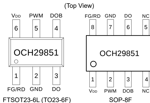
Figure 1, Pin Assignments of OCH29851
