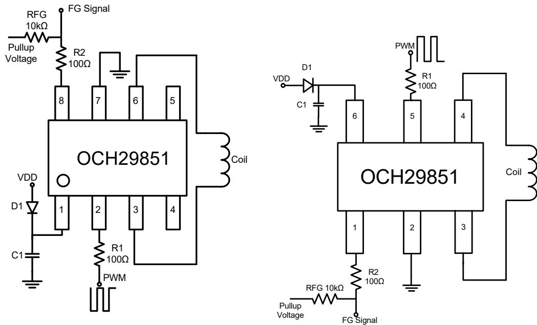
Figure 2, Typical Application Circuit of OCH29851
