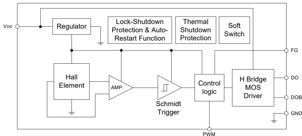
Figure 3, Block Diagram Of OCH29851
